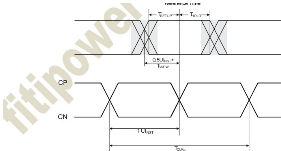
Figure 11.6: Data to Clock Timing Definitions
