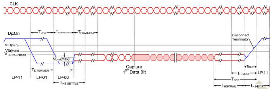
Figure 11.7: High-Speed Data Transmission in Bursts
