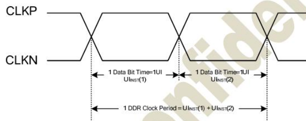
Figure 11.5: DDR Clock Definition
