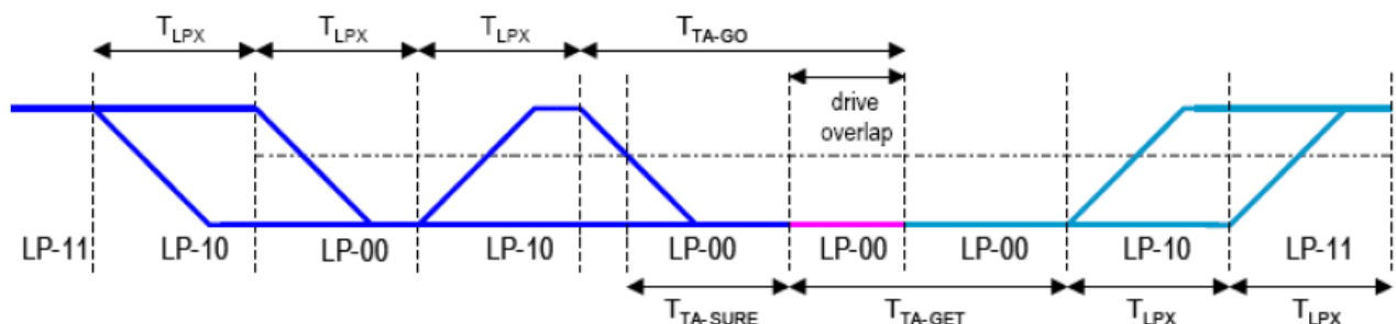
Turnaround Procedure
